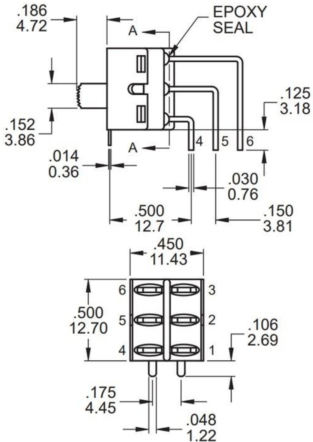
Section drawing for A-A.
